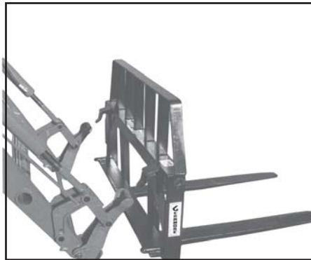
Fig. 4 Alignment
