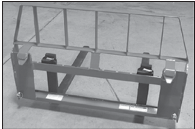
Fig. 3 Mounting with John Deere Quick Coupler
