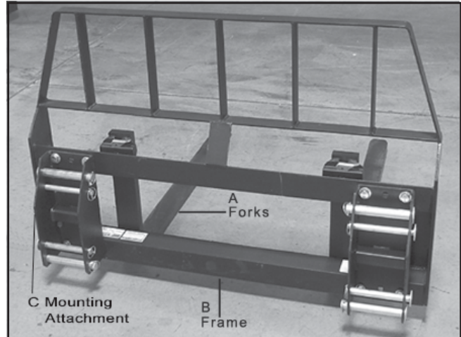
Fig. 1 Machine Components
