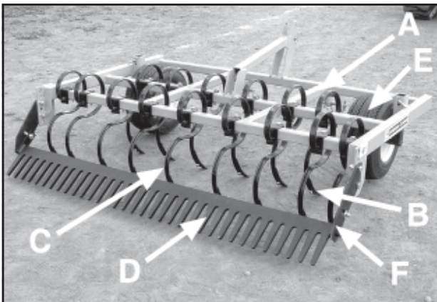
Fig. 1 - Machine Components
