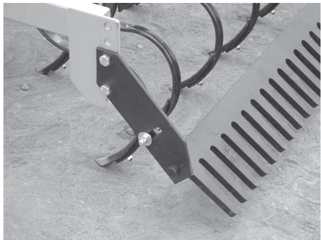
Leveling Comb Angle
