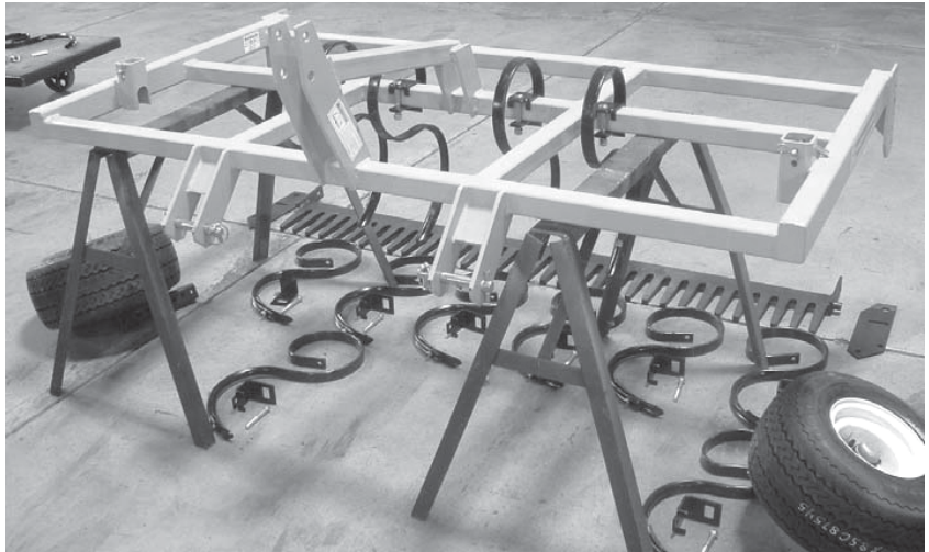
Fig. 13 - 3-Point Hitch Mounts
