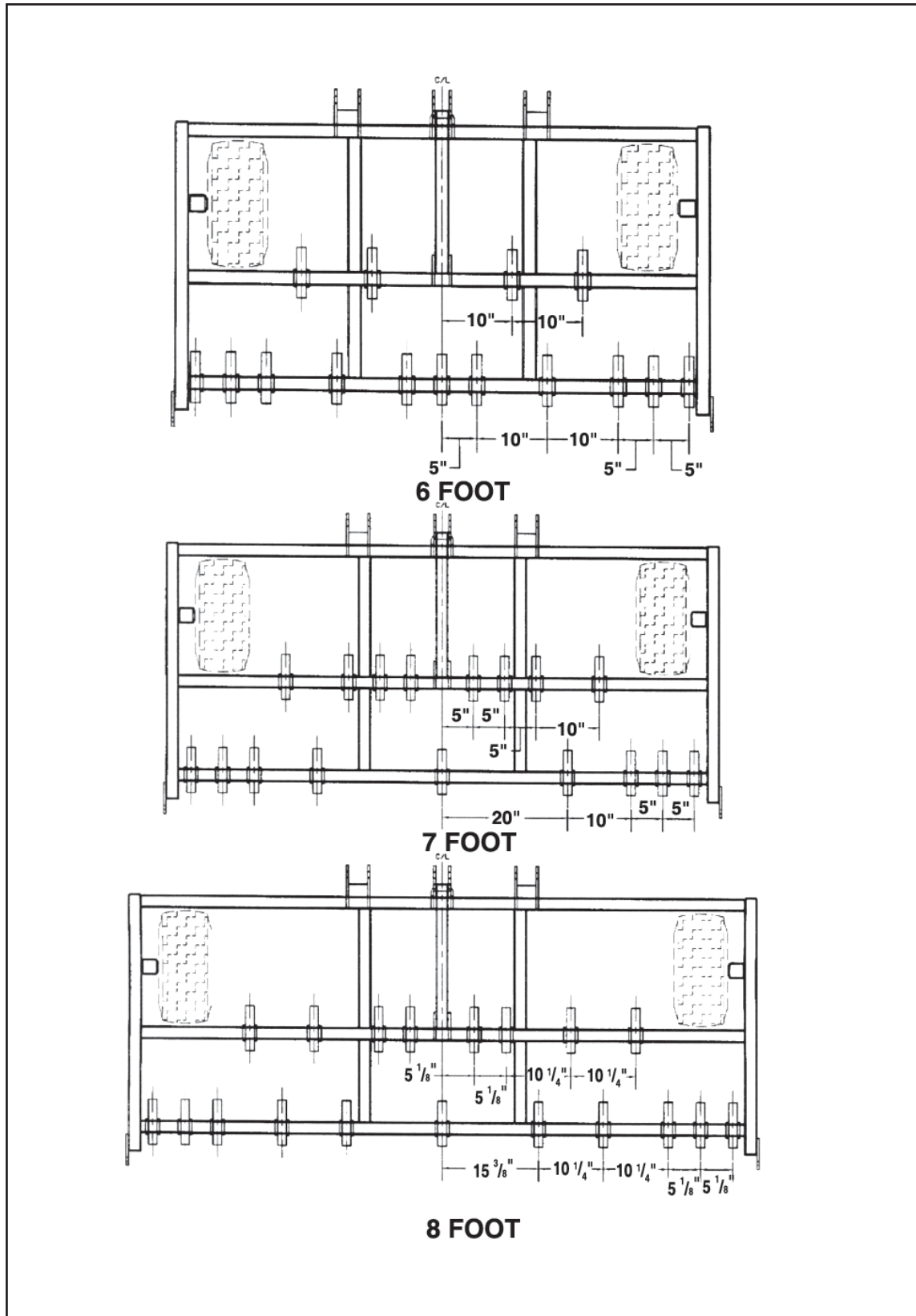
Fig. 12 - Tine Positions
