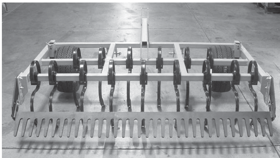
Fig. 17 - Assembled
