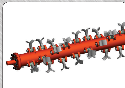
Rotorshaft with heavy swing Y blades
