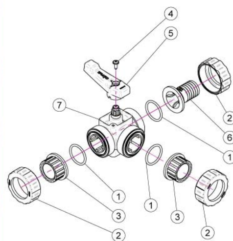
3-WAY VALVE
