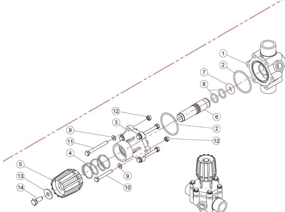
PRESSURE REGULATOR
