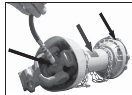
Figure M-2 U-joints
