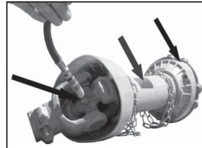
Figure M-2 U-joints
