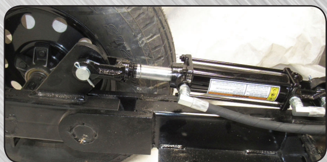
Hydraulic tilt with hoses
