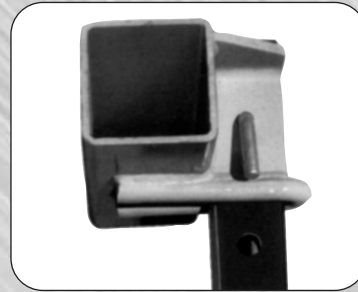
Special High Strength Shank Pockets
