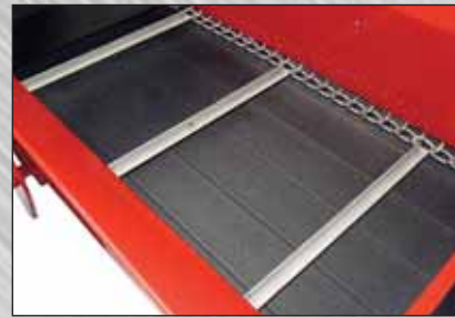
Stainless Steel T-rod apron chain and poly floor
