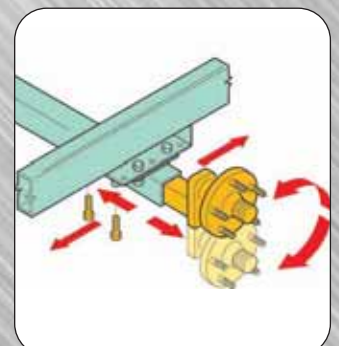
Wheels adjust up or down, in or out, front or rear to obtain best balance and clearance
