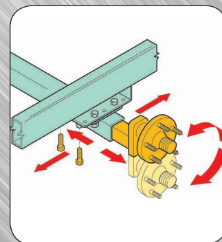
Wheels adjust up or down, in or out, front or rear to obtain best balance and clearance
