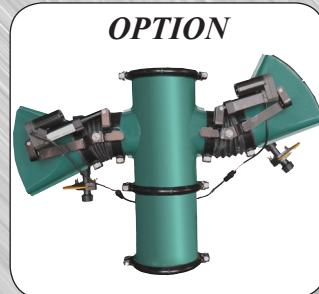
OPTION Electro cylinders on narrow row fishtail spray heads, with 32 orifice outlets
