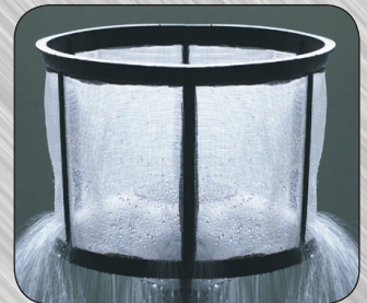
Shower head is built into the main strainer basket to easily put wettable powders into suspension
