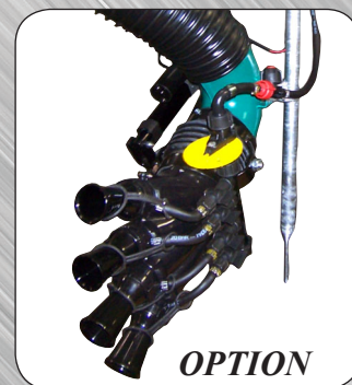
OPTION Electro cylinders with control box operated from tractor seat (outer spray heads)
