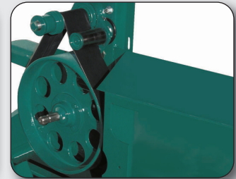
Power band fan speed up system with built-in overrunning clutch
