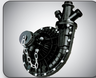
Low pressure centrifugal pump made of anti-corrosive materials requires little maintenance
