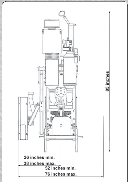
Leaf Remover Dimensions
