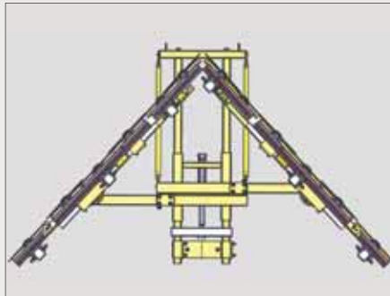
DOUBLE CROSSARM TRELLIS SYSTEM
