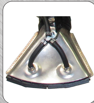
Stainless steel "Fishtail" nozzles with 16 spray outlets
