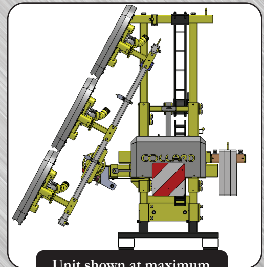
Unit shown at maximum tilt of 28 degrees
